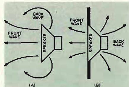
A) Back and front waves conflict in unbaffled speakers. B) In mounted speakers, the "baffle" keeps them apart.
