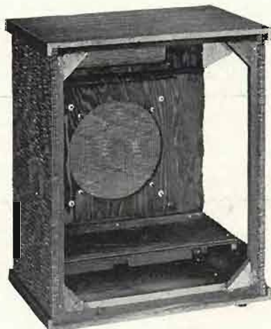
Bass reflex: the back wave turns around to reinforce the low notes.
