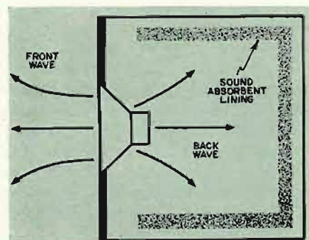
Infinite baffle: the back wave is absorbed by the lining of the box.
