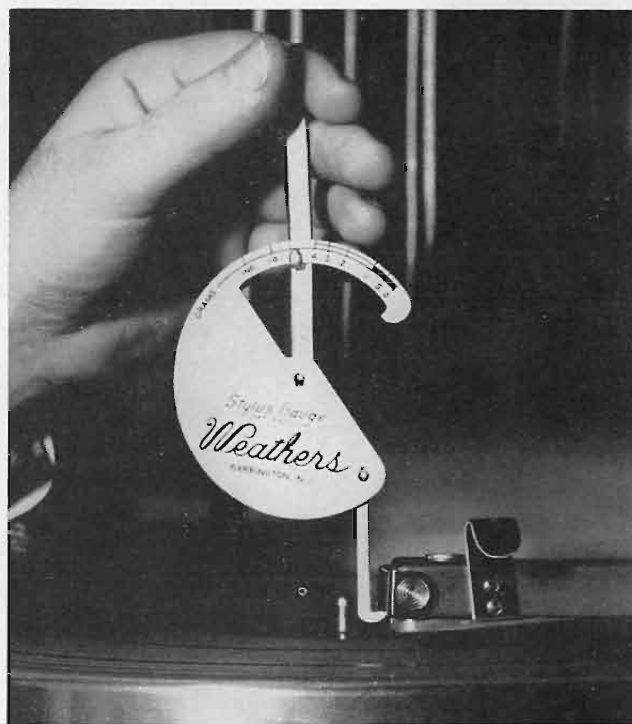
The Weathers scale is basically a counter-balanced lever while the Clarkstan stylus pressure gage works by deflecting a spring.
