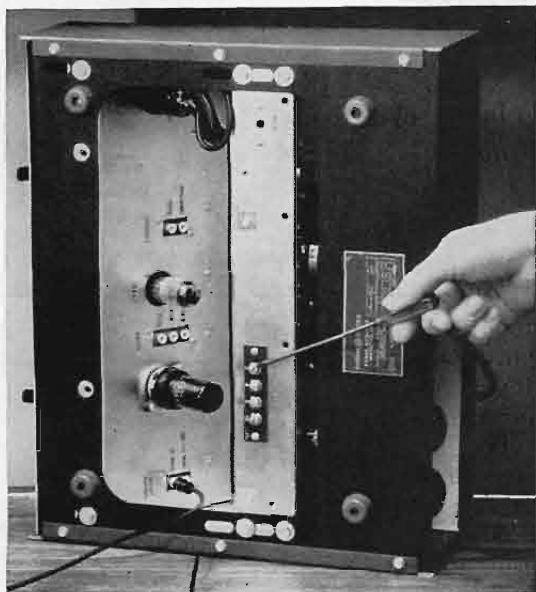
Access to output, input and loudspeaker connections necessitate turning PA-20 on its side. Hum level control is visible.
