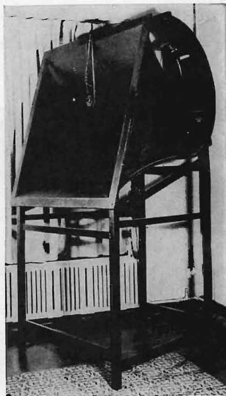
An early coaxial. Note tiny tweeter suspended across woofer horn mouth.
